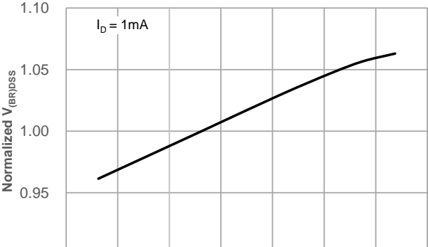
Figure 11: Normalized Breakdown voltage vs. Junction Temperature
